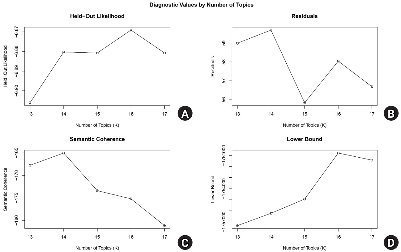
Supplementary Figure 2. (A-D) Diagnostic values by number of topics (K=13 to 17).
